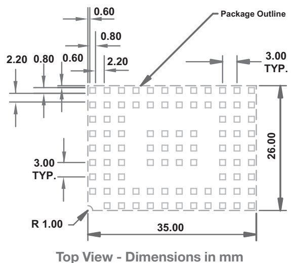
Figure 9 Package Dimensions
