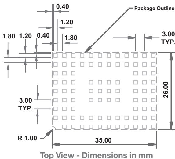
Figure 8 Footprint Dimensions
